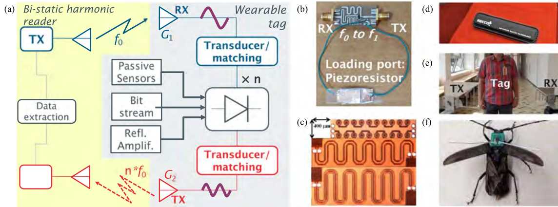
FIGURE 8. Harmonic backscattering systems approaching wearable applications: (a) operation principle [10]; (b) a sensor-loaded PCB modulator [?] Bsemi BIparcBrpar fully-integrated harmonic transponder [102] (IEEE 2010); (d) a commercial avalanche rescue RECCO™ tag based on harmonic backscattering; (e) off-body interrogation of a wearable harmonic tag [103]; (f) “wearable” harmonic tags for insect tracking [104] (IEEE 2020).
